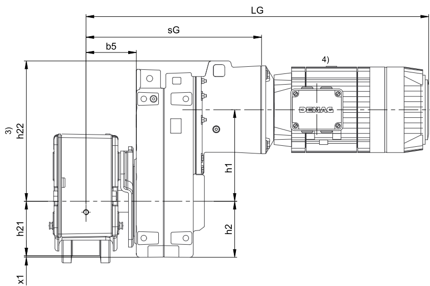
AD 70 - AD 80 2/3-stufig
